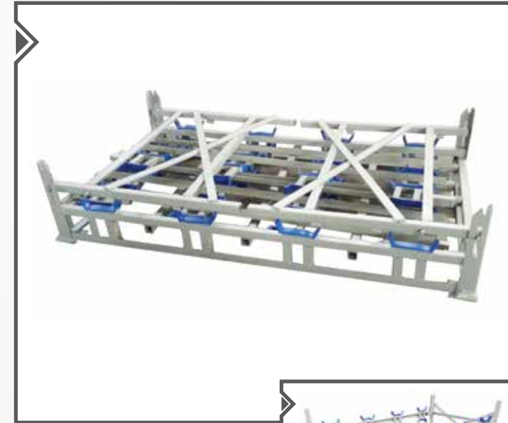
62 DİNGİL PALETİ / PALLET FOR AXLE
